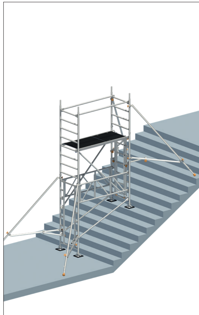
16. Attach the stabilisers (see p. 20, Section 7, Stabiliser Attachment)
