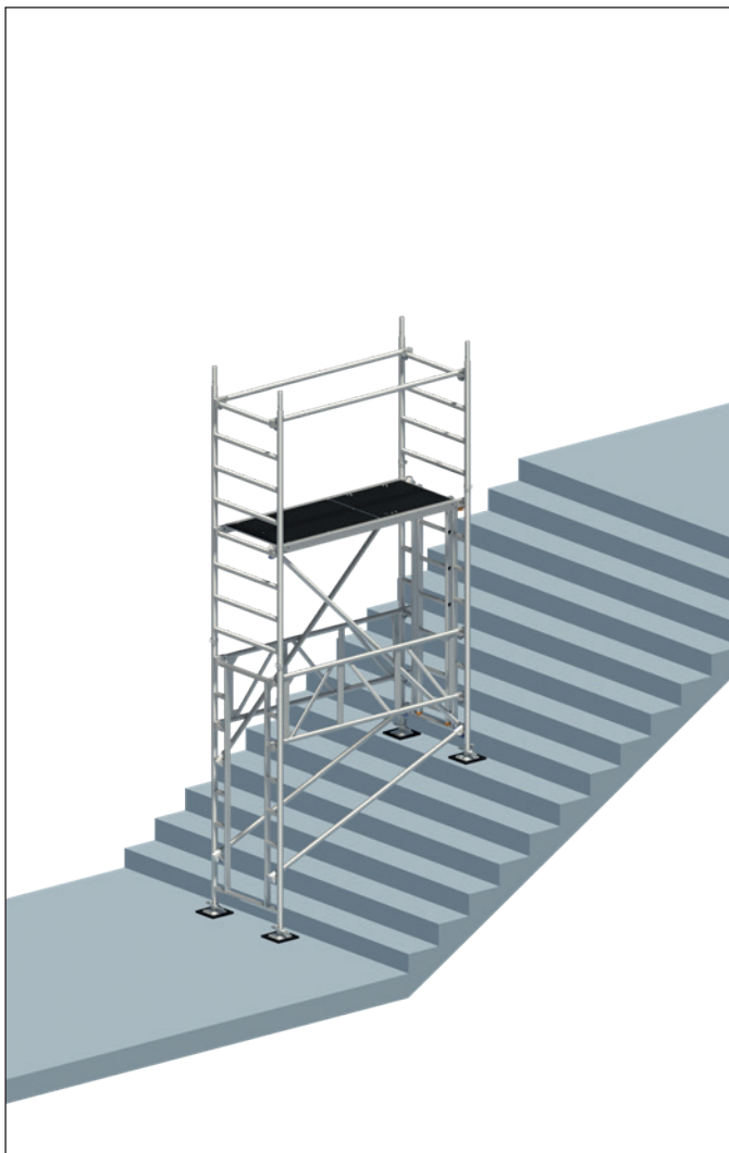
15. Fit the suspended ladder 10 (see p. 21, Section 8, Suspended Ladder Attachment) for safer upward access.
