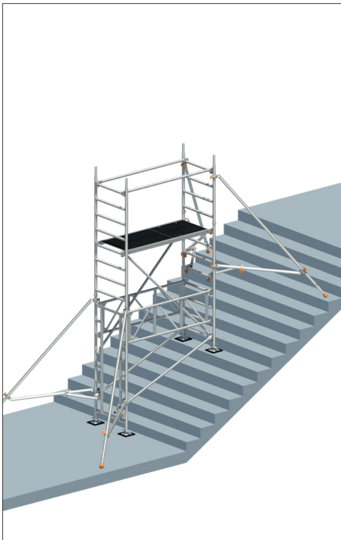
15. Attach the stabilisers (see p. 20, Section 7, Stabiliser Attachment)
