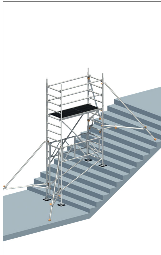
16. Fit the guardrails at the 50 cm level.
