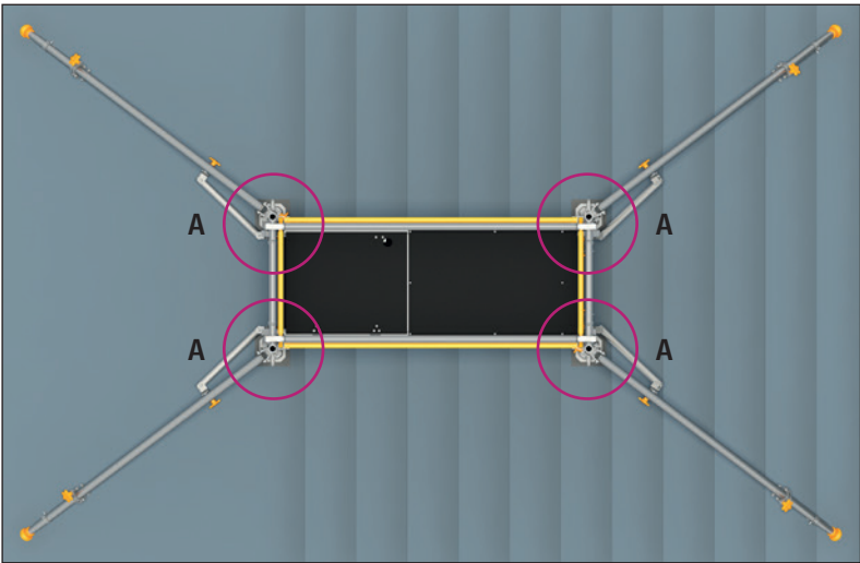
Ballasting table for Variant 3
